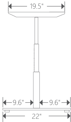
2-Leg Small Frame [UP-2LS] Side View
