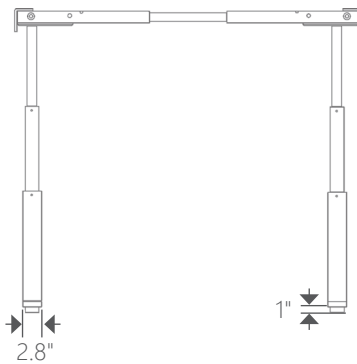
Front View On All Frames
